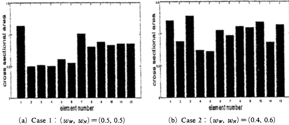
Fig. 3 Distribution of cross sectional area
