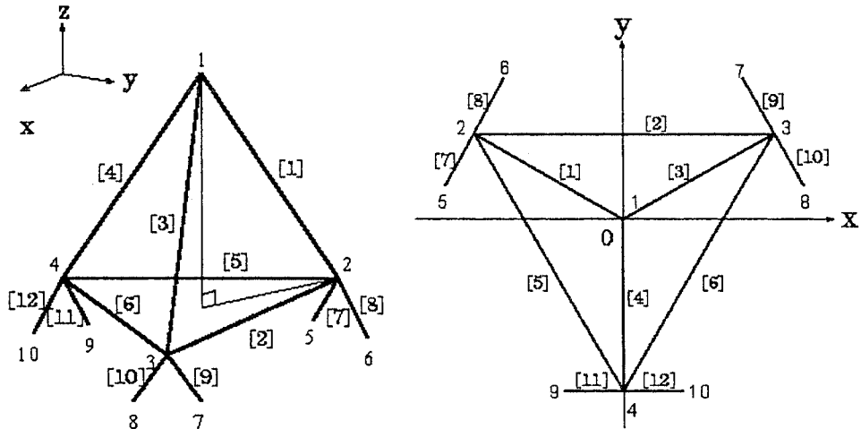
Fig. 2 3-D truss structure
